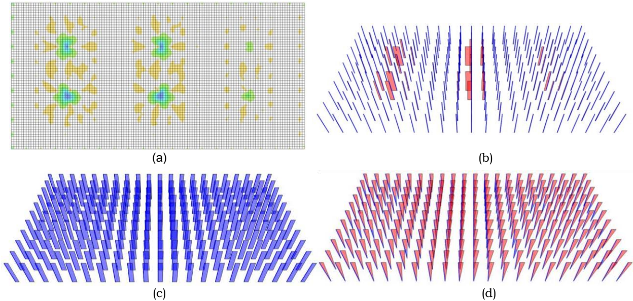
Figure 11: Internal forces in the sample system calculated under the truck load effect
